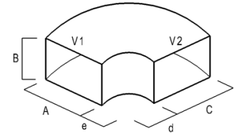
Normradius r = 120 mm
